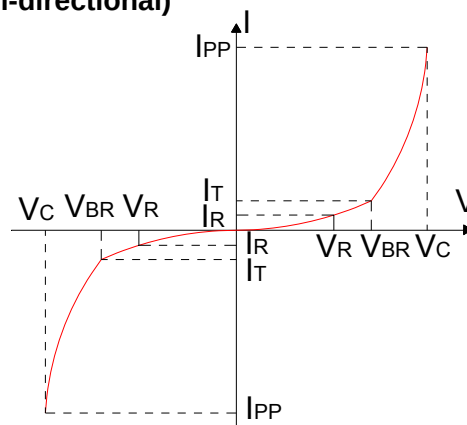
FIG.2:V- I curve characteristics (Bi-directional)
